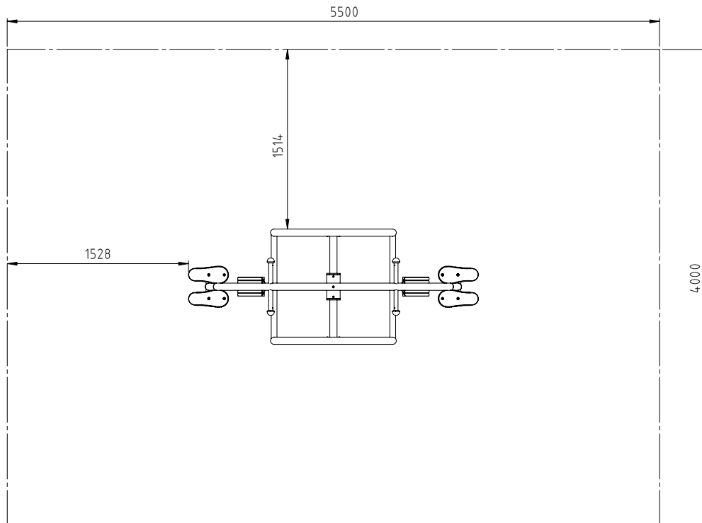
Diagram 3: Top view
