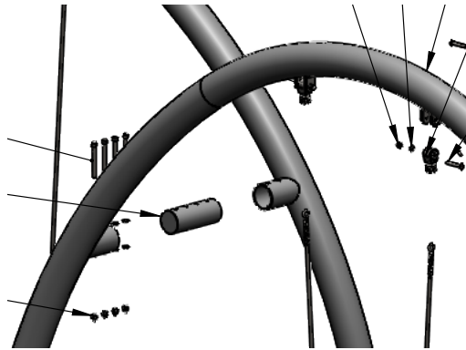
Diagram 4: Connection of the two parts of the swing
