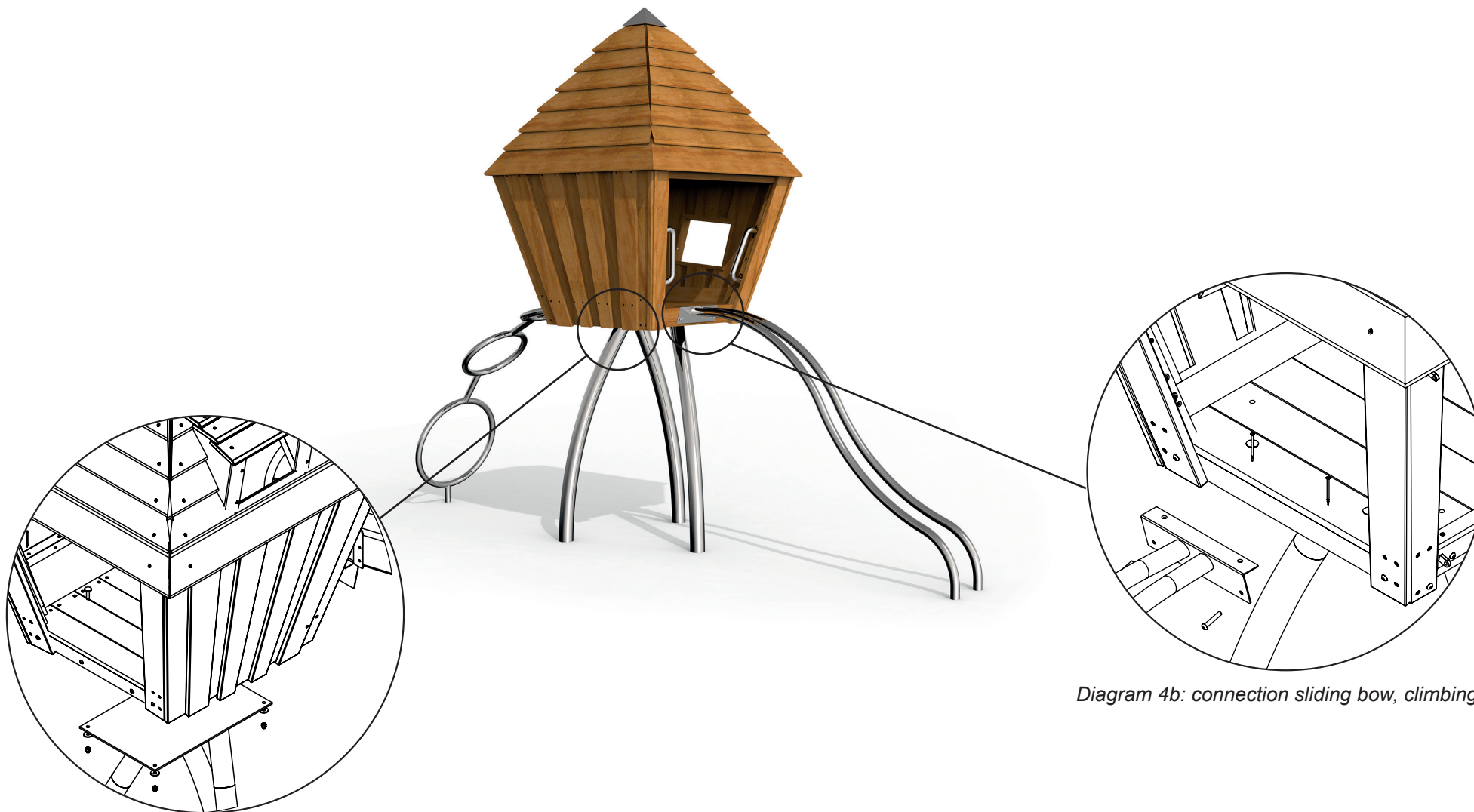
Diagram 4a: connection wendy house
