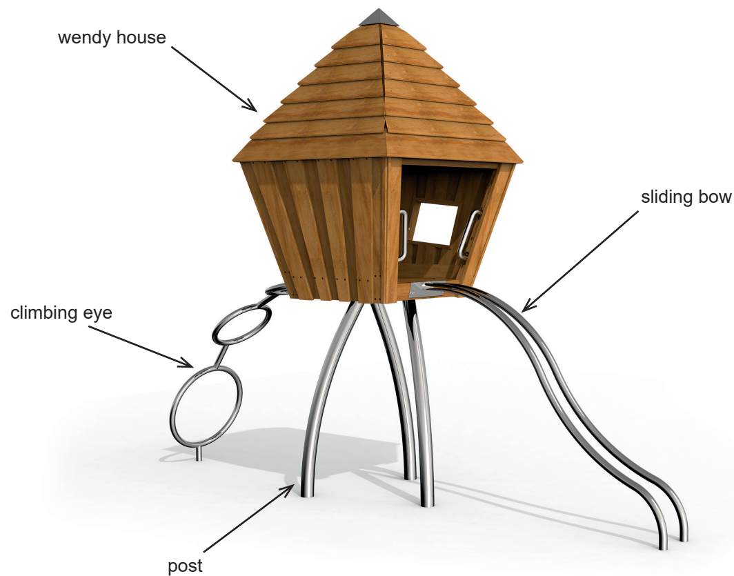
Diagram 1: Overall view of the play equipment
