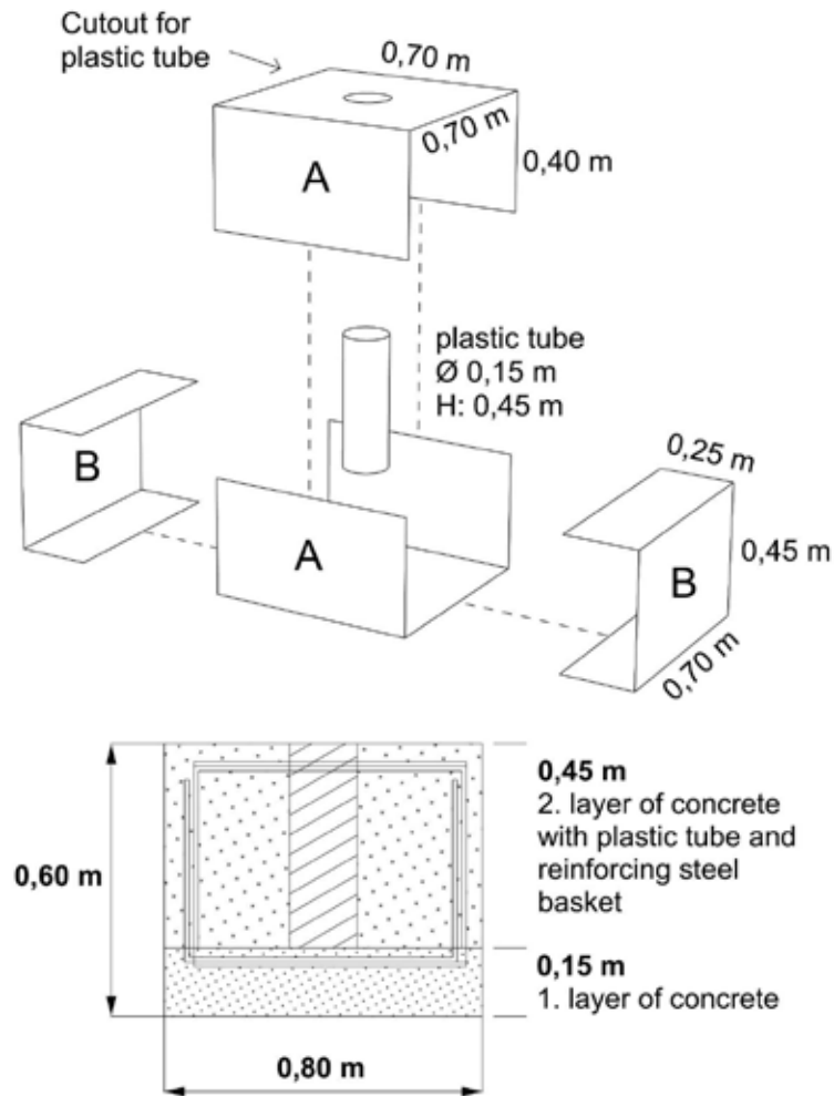
Diagram 2: Production and position of the reinforcement basket for the middle foundation
