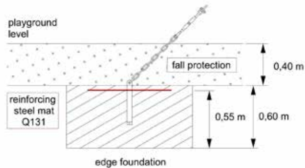
Diagram 3: Construction of the foundation with a reinforcing steel mat
