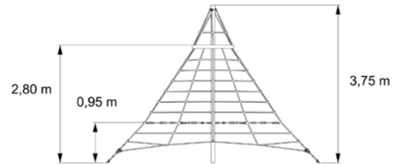
Diagram 8: Front view with net level
