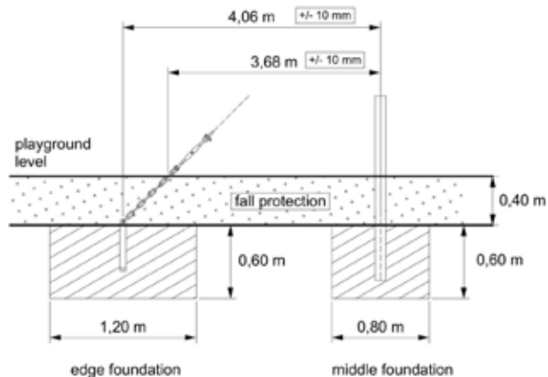
Diagram 4: Distance between the foundations and in the device space
