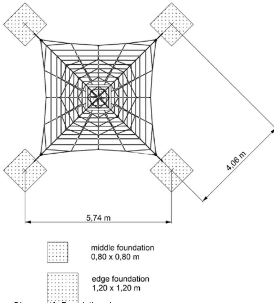
Diagram 10: Foundation plan
