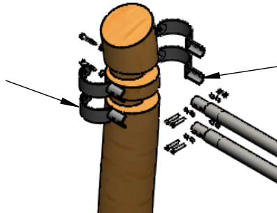
Diagram 4: Assembly
