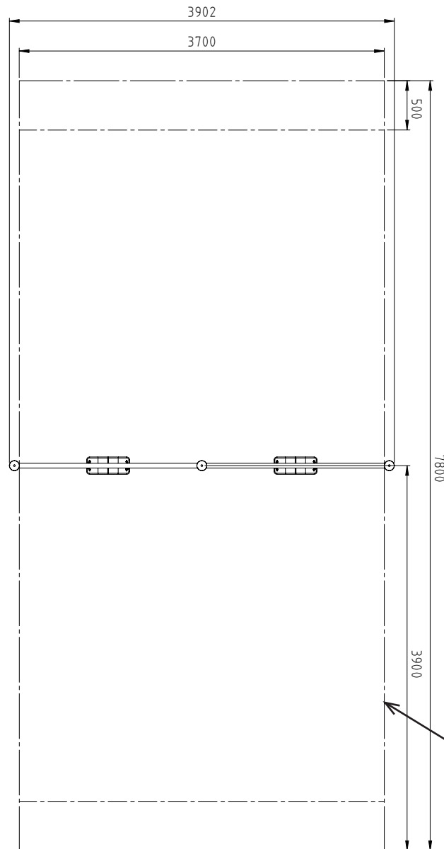
Diagram 4: Top view
