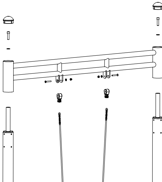
Diagram 3: Assembly
