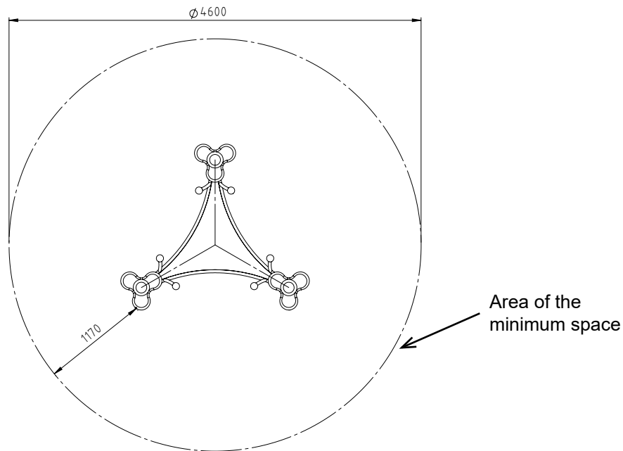
Diagram 3: Top view
