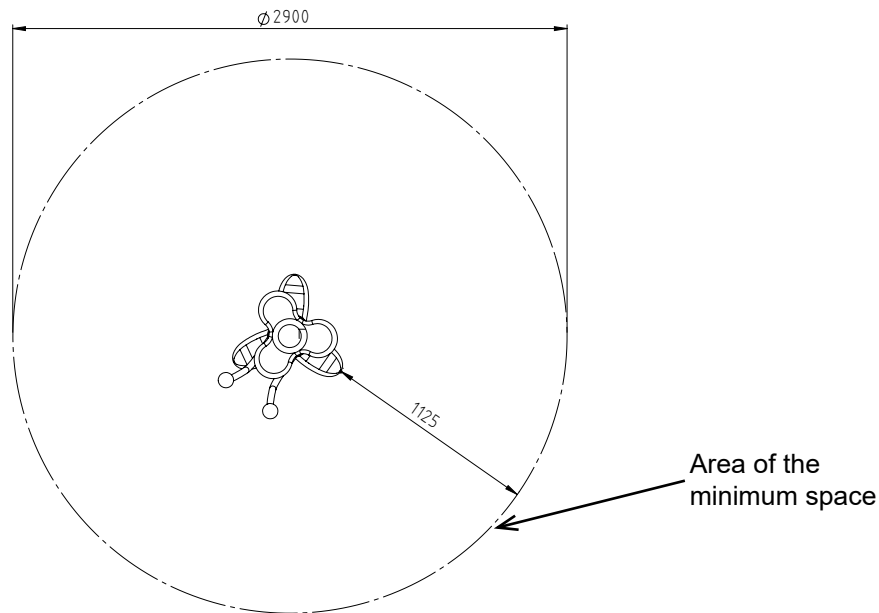
Diagram 3: Top view
