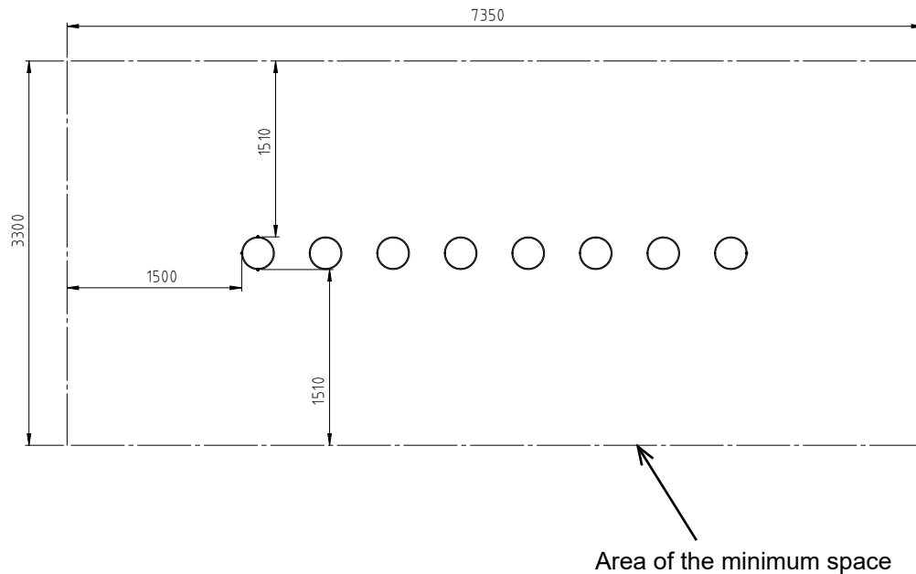
Diagram 3: Top view
