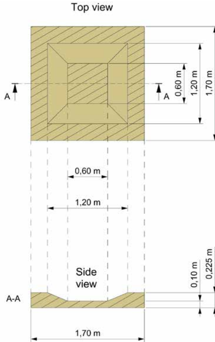
Diagram 2: Combined frost protection and load bearing layer
