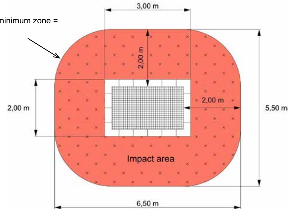
Diagram 4: Top view
