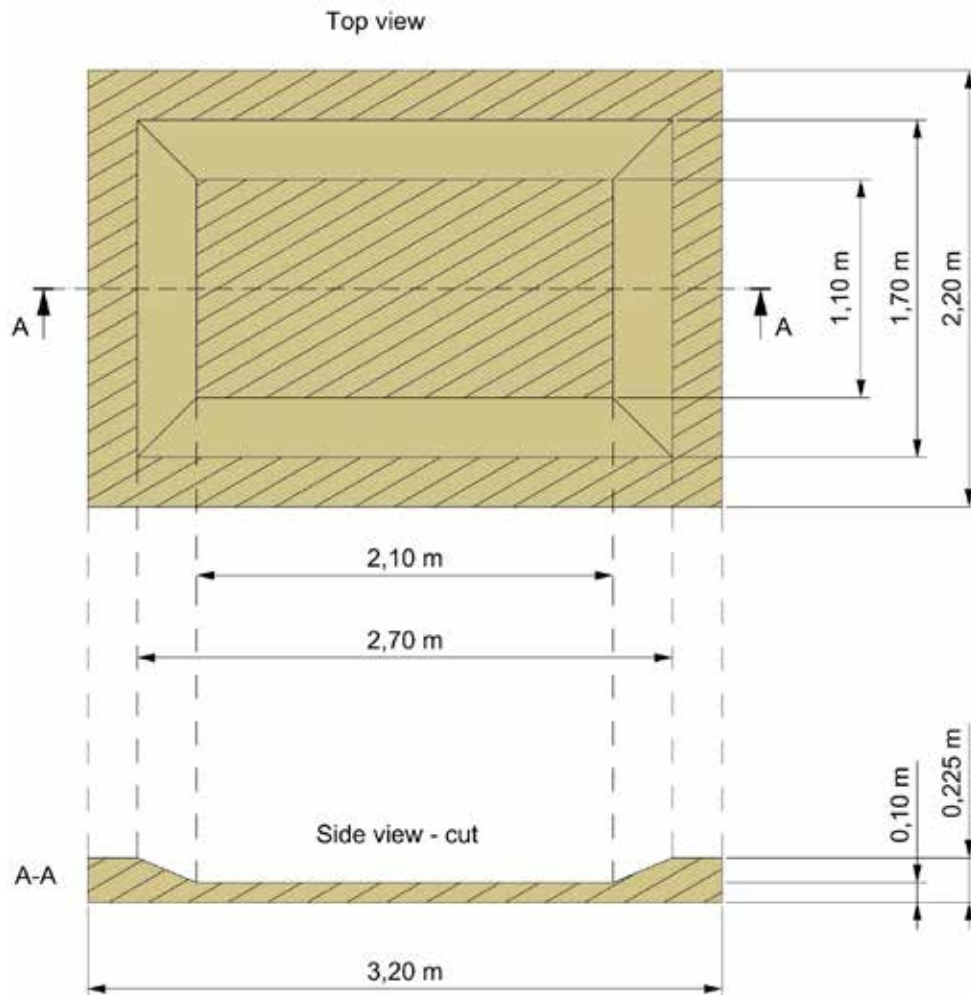
Diagram 2: Combined frost protection and load bearing layer
