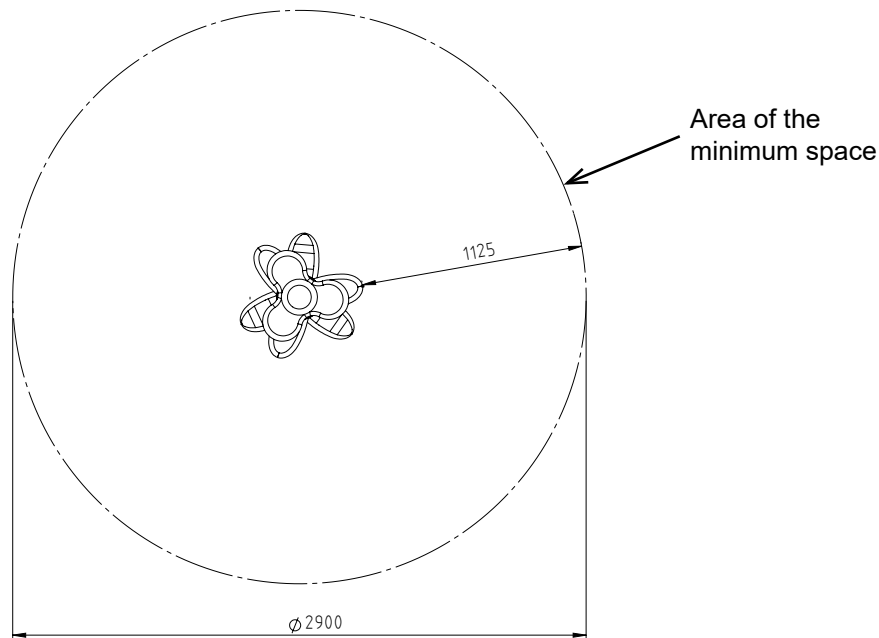
Diagram 3: Top view
