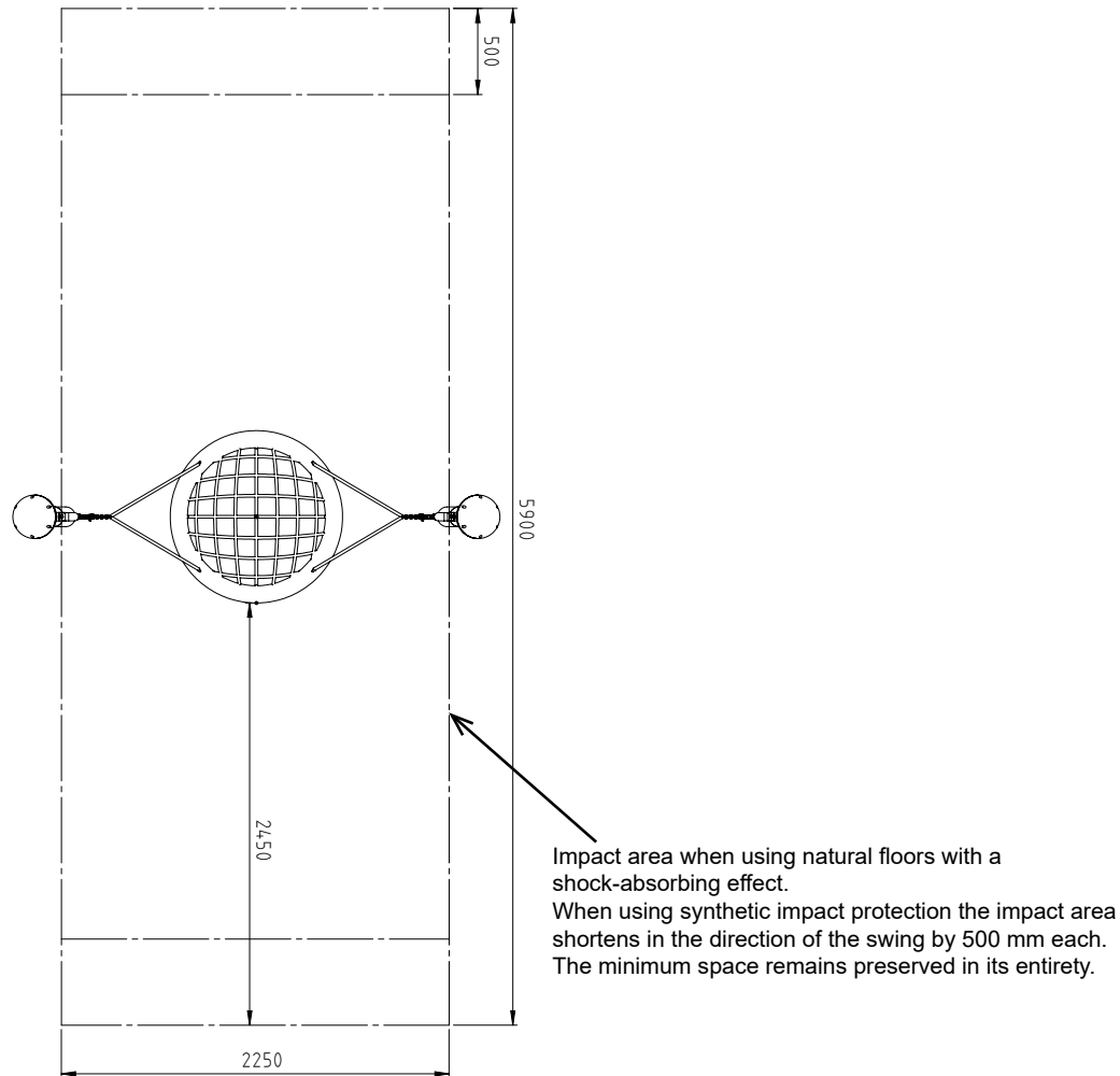
Diagram 3: Top view
