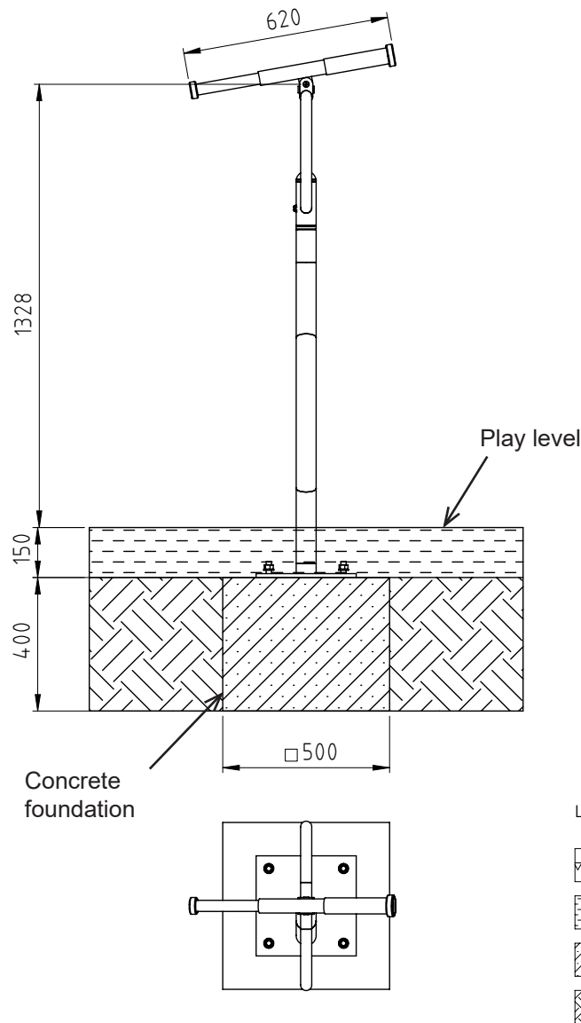
Diagram 2: Foundation plan
