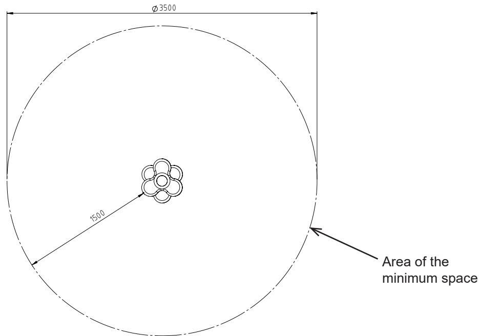
Diagram 3: Top view
