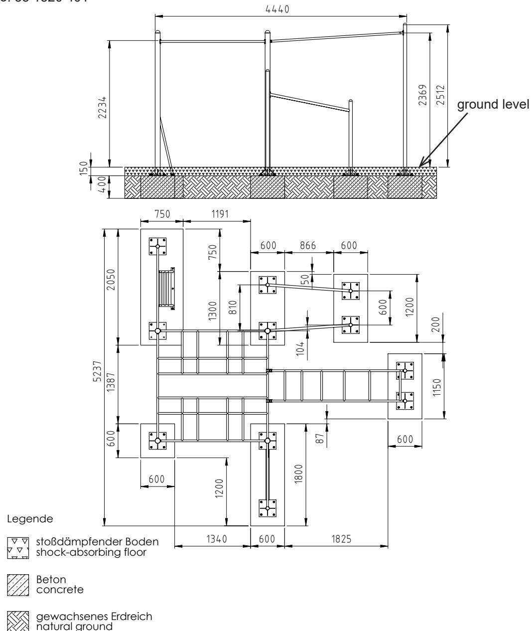
Diagram 2: Foundation plan
