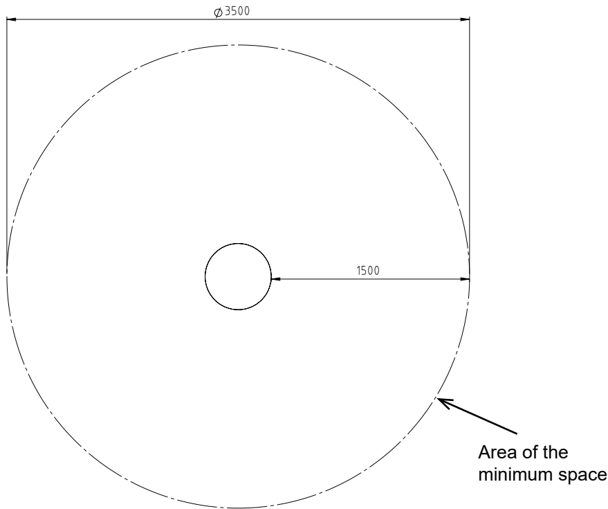
Diagram 3: Top view
