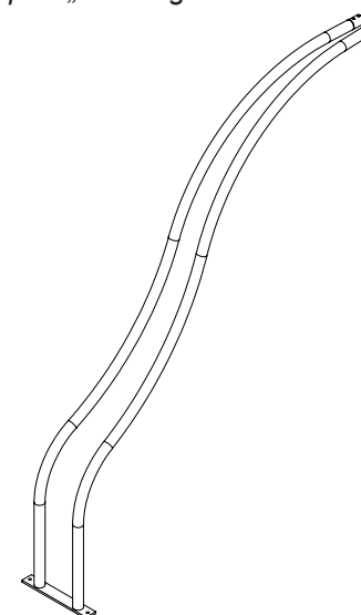
Diagram 5c: attachment part „sliding bow“
