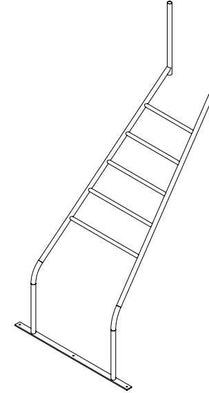
Diagram 5a: attachment part „climbing slant“
