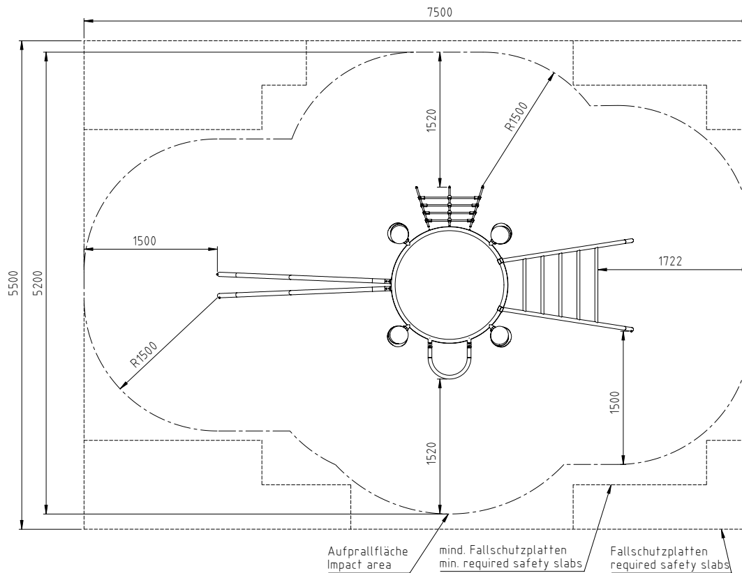
Diagram 3: Top view
