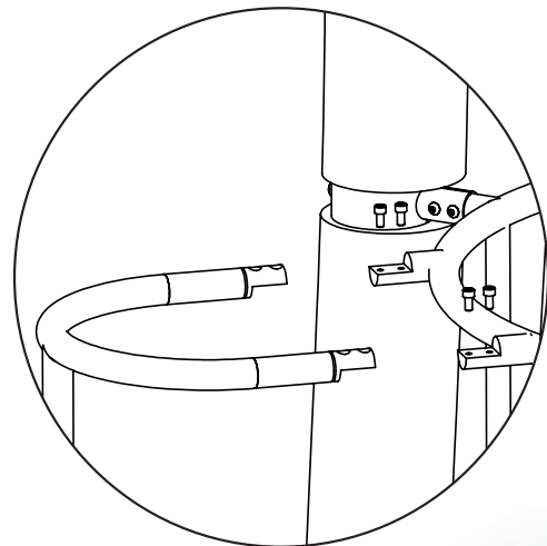
Diagram 5a: connection firemans pole
