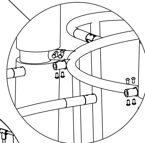
Diagram 5e: connection climbing arc
