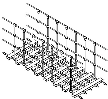
Diagram 4d: attachment part „wobble bridge“
