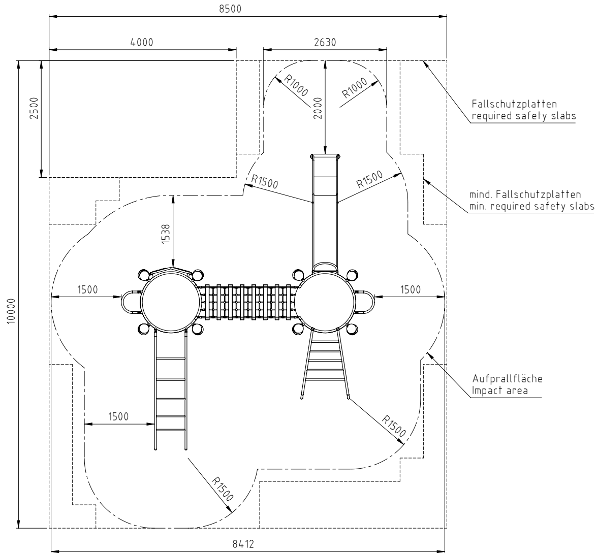
Diagram 2: Top view
