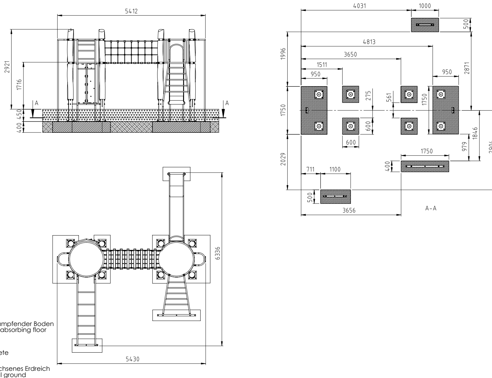
Diagram 3: Foundation plan
