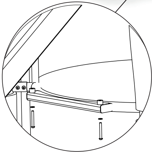
Diagram 5b: connection slide
