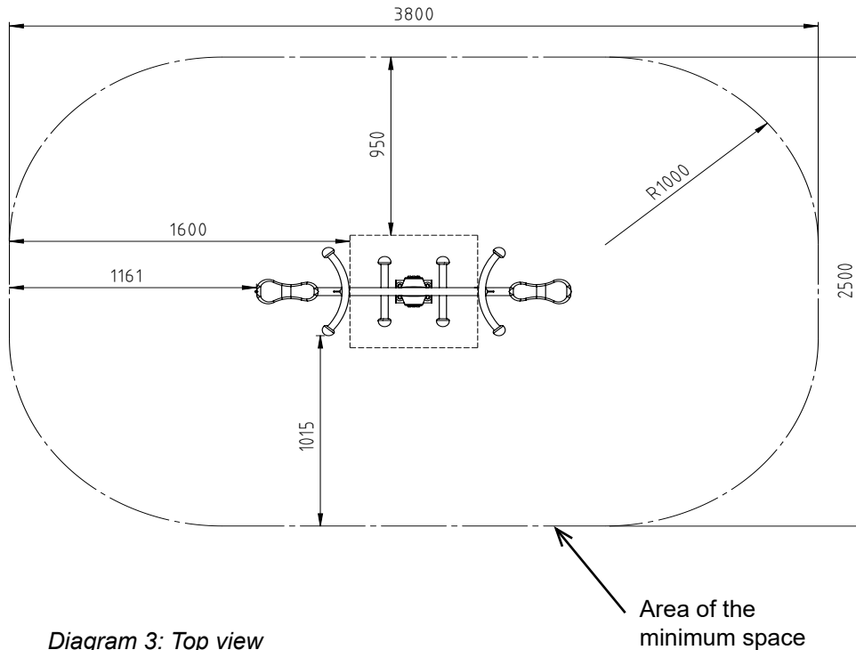
Diagram 3: Top view
