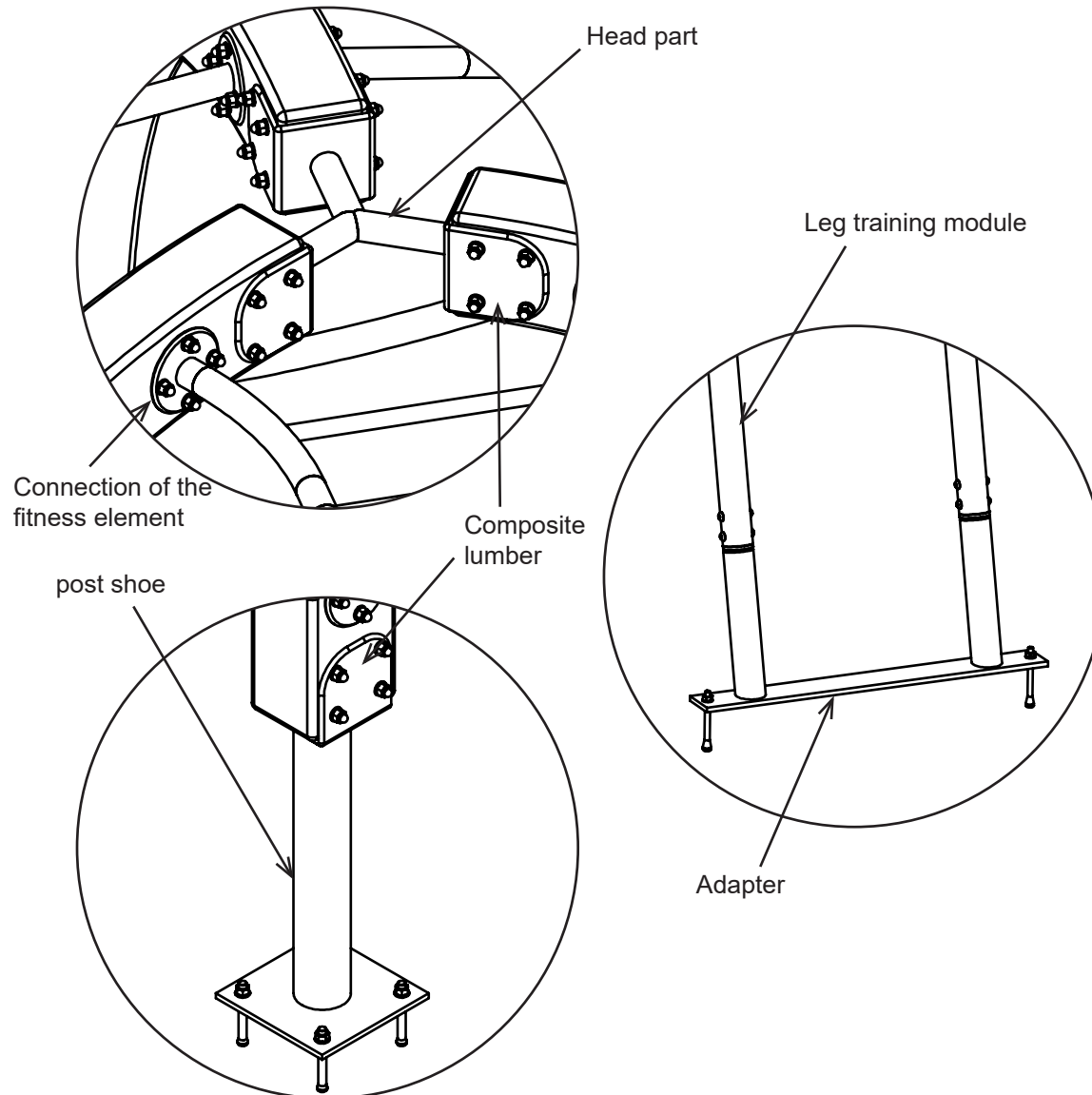
Diagram 3: Detailed elements
