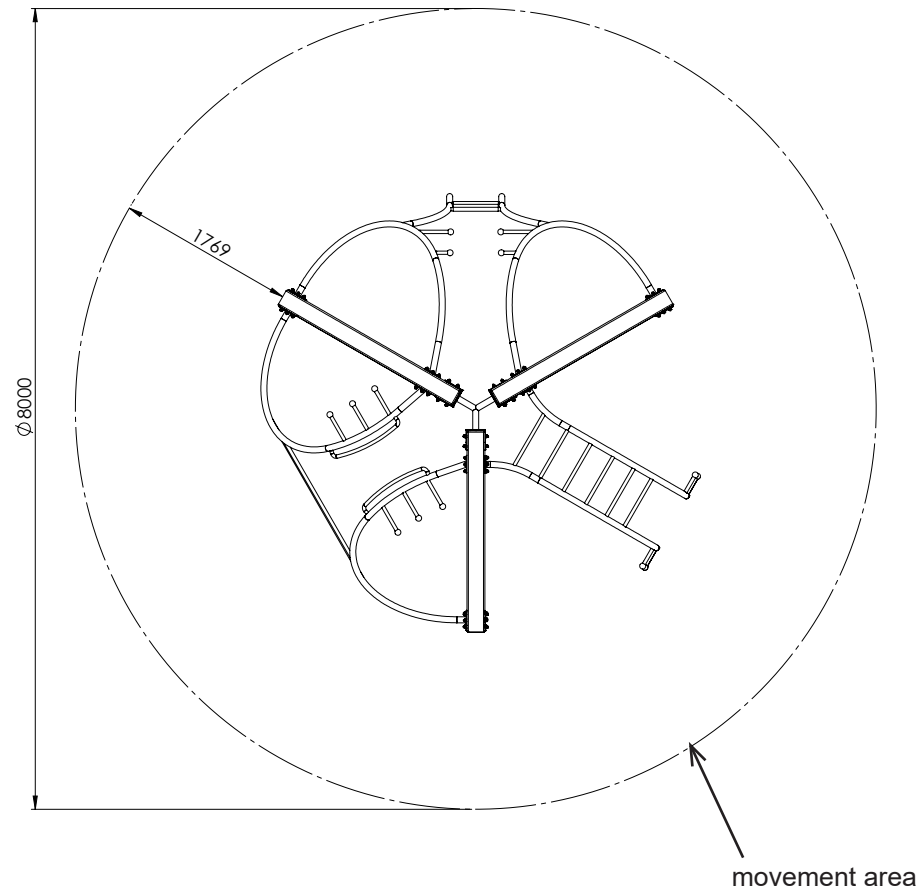
Diagram 4: Top view
