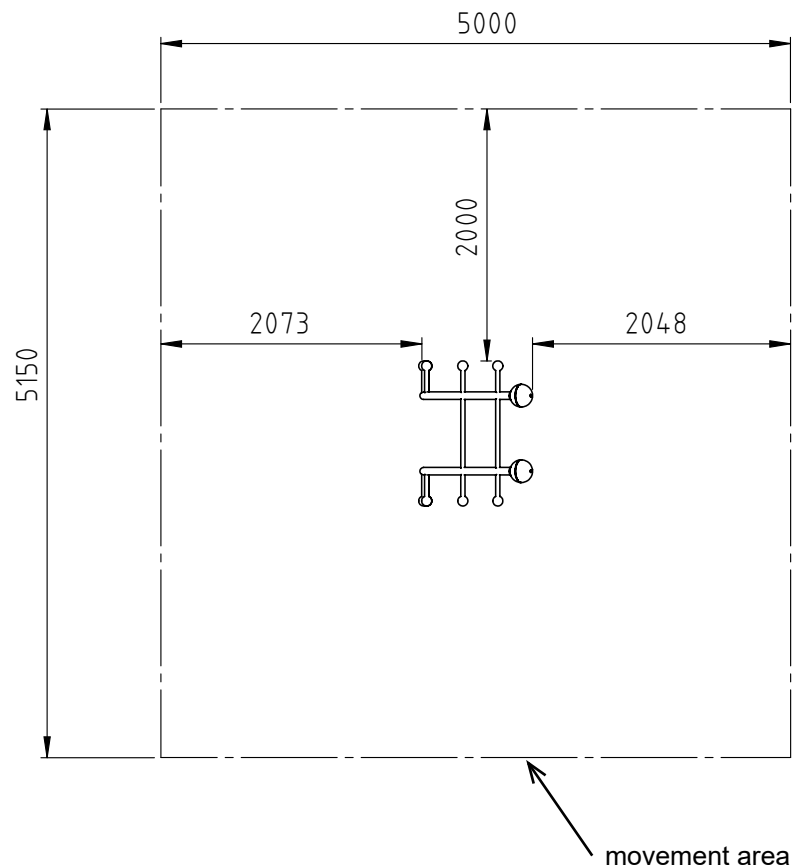
Diagram 3: Top view
