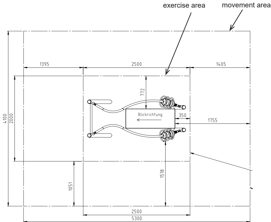
Diagram 3: Top view
