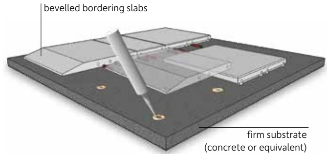
Laying (staggered) on a level, solid surface with bevelled edge slabs & system plugs. Bonding with gluing spots on the drainage.
