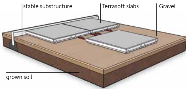
Laying (staggered) on permeable substrate (lava, basalt, gravel, grit) with edging element and system plugs.
