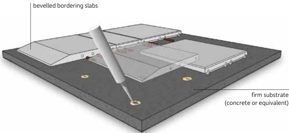
Laying (staggered) on a level, solid surface with bevelled edge slabs & system plugs. Bonding with gluing spots on the drainage.
